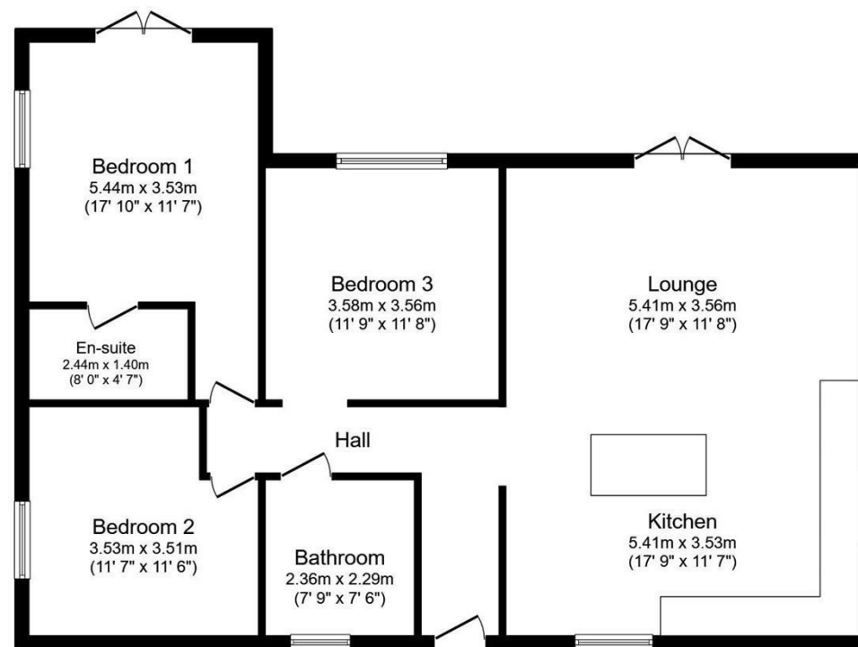
Floor Plan
